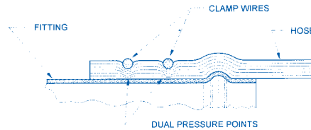
Double Sealing Action
